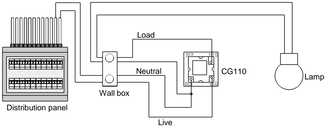
Situation 1: Live , Neutral and Load wires are ready at wallbox
